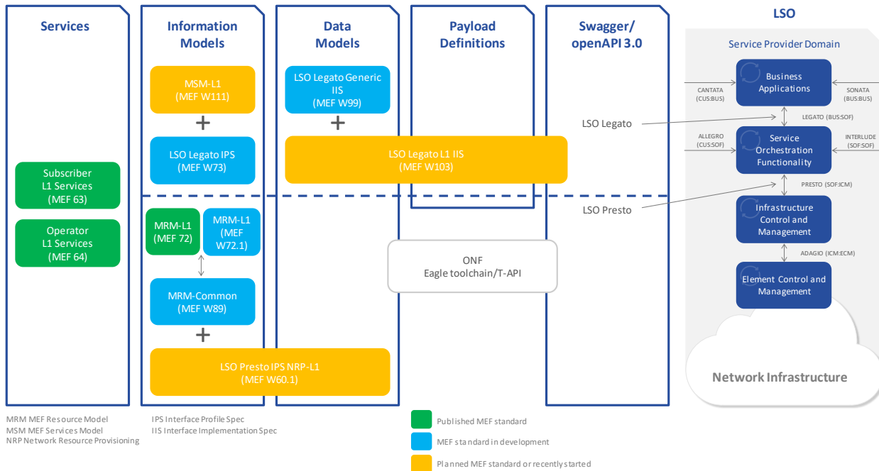
Figure 8 – LSO-Related Specifications for MEF 63 and MEF 64
