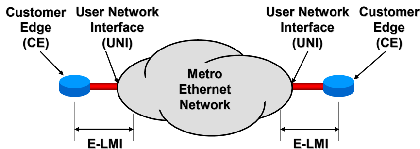
Figure 1 – E-LMI Scope
